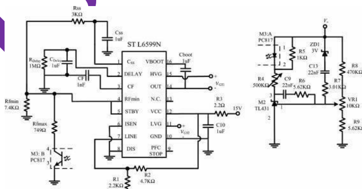
Fig. 5. Control circuit.
